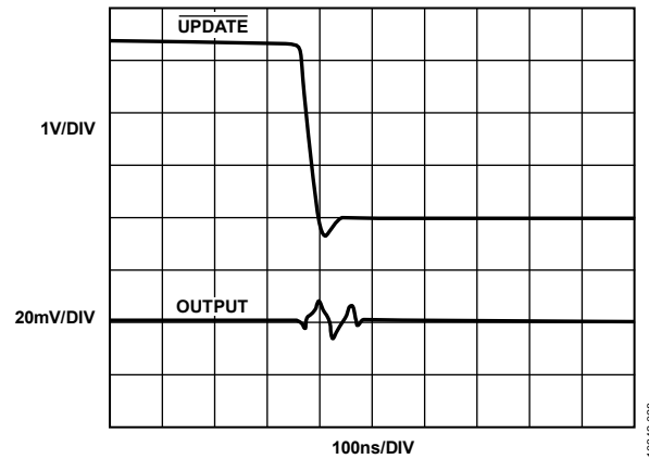
Figure 23. Switching Transient
